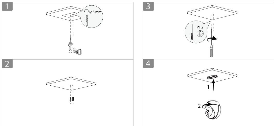
Figure 3-5 Ceiling mount
